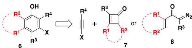
Scheme 2. Benzannulation Disconnection for Polycyclic Compounds
